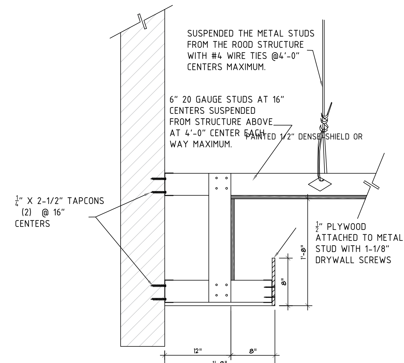
⑤ DRYWALL CEILING STRUCTURE DETAIL SCALE: 1-1/2" = 1'-0"
