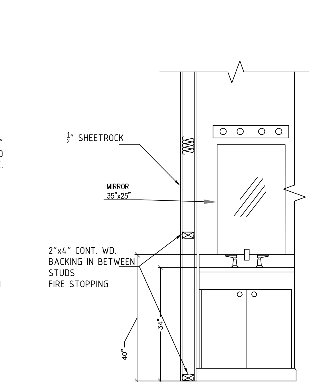
⑫ TYP. KITHEN DETAIL SCALE: 3/4" = 1'-0"
