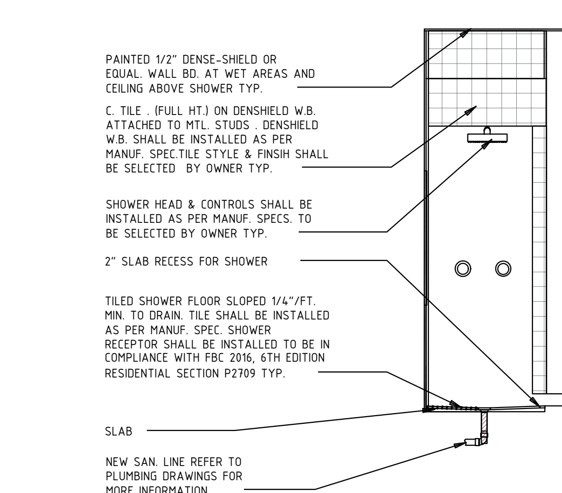
⑩ TYP. SHOWER DETAIL SCALE: 1/2" = 1'-0"
