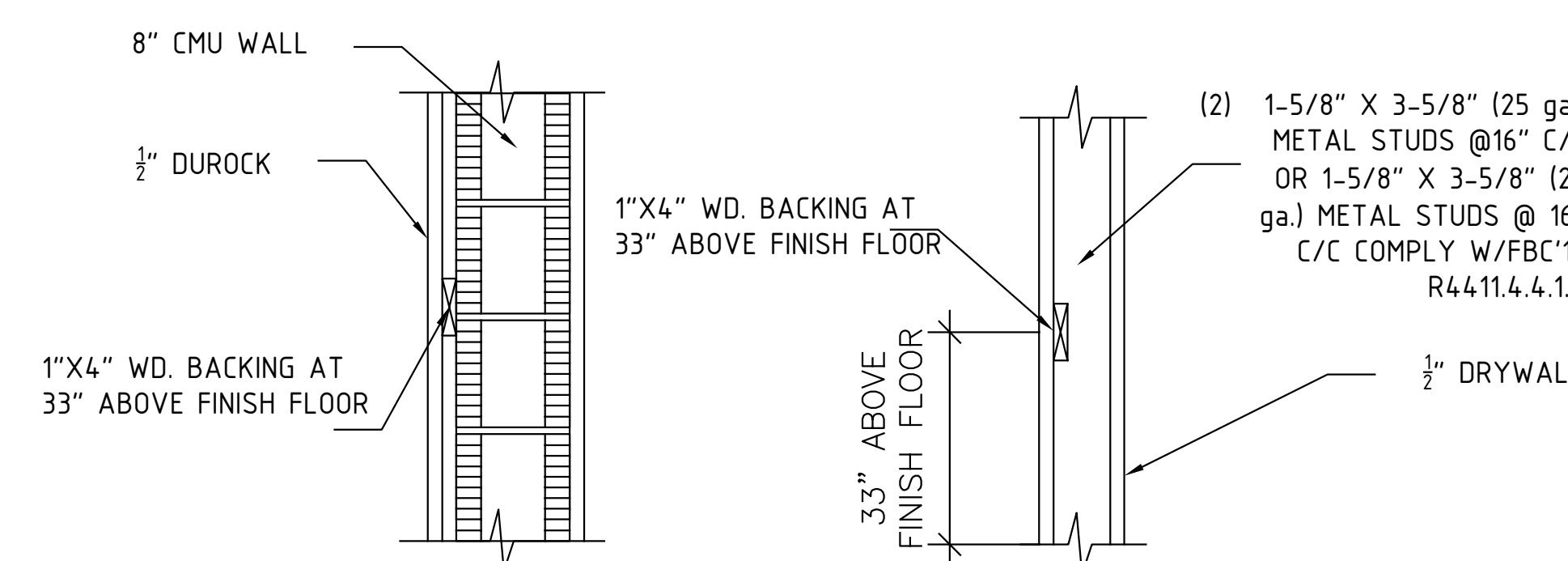
⑧ BATHROOM BACKING DETAIL SCALE: 1/4" = 1'-0"
