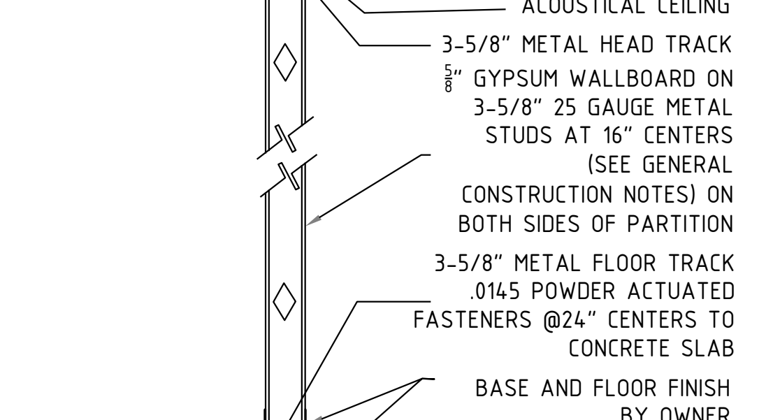
⑧ TYPICAL LOW PARTITION SCALE: 3/8" = 1'-0" (NON-BEARING, NON- FIRE-RATED)
