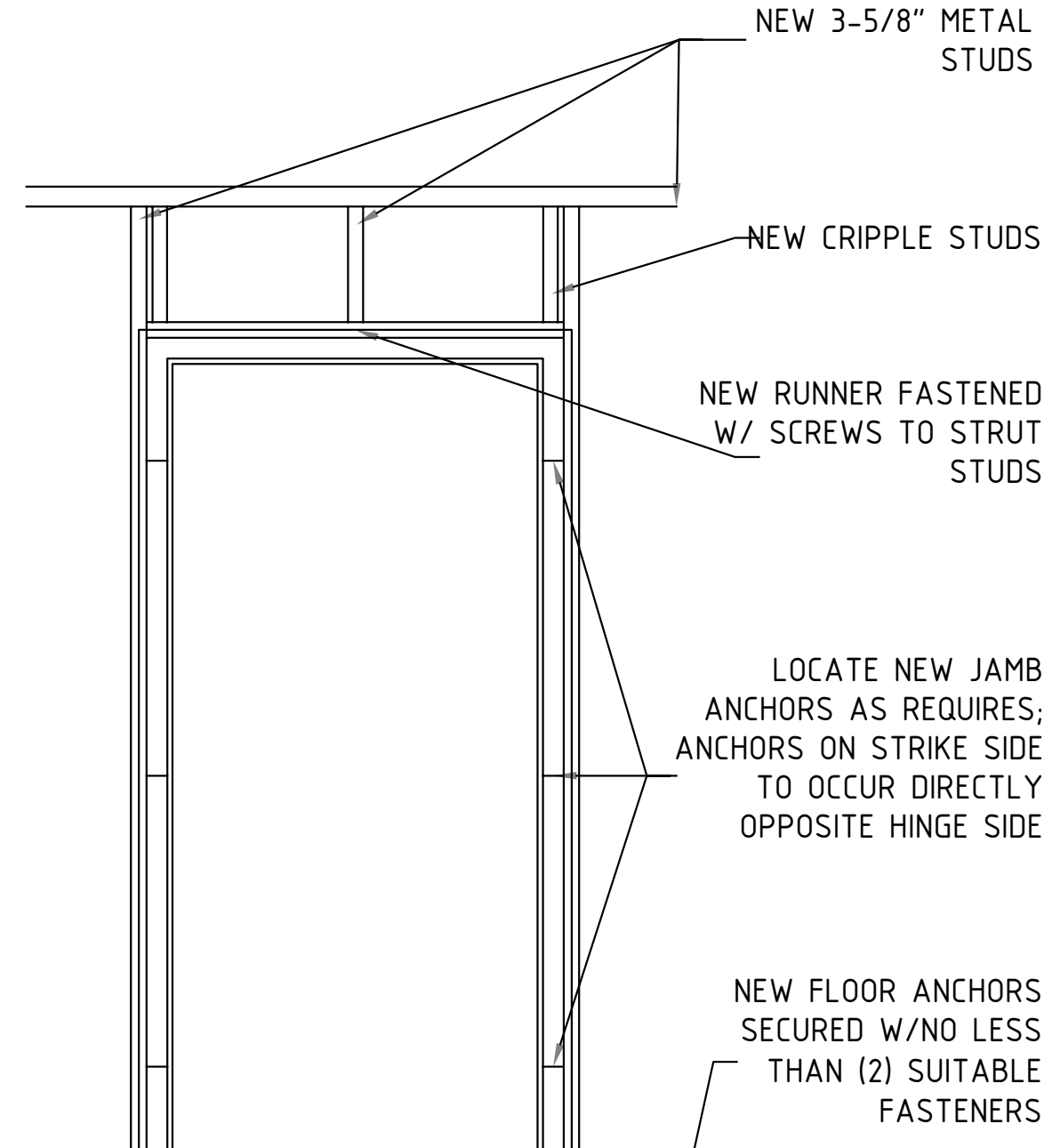
⑦ TWO SIDED LIGHT COVE DETAIL SCALE: 1/2" = 1'-0"
