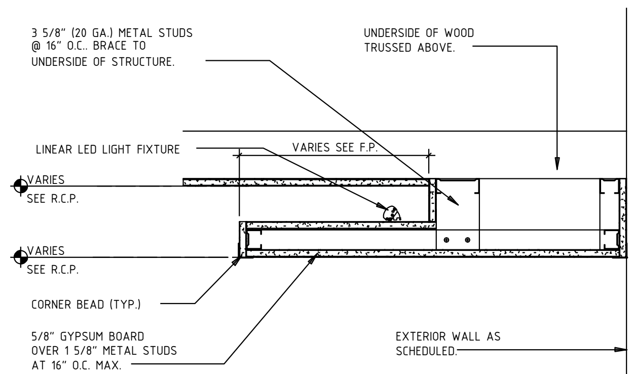
② TYPICAL LIGHT COVE DETAIL SCALE: 1 1/2" = 1'-0"
