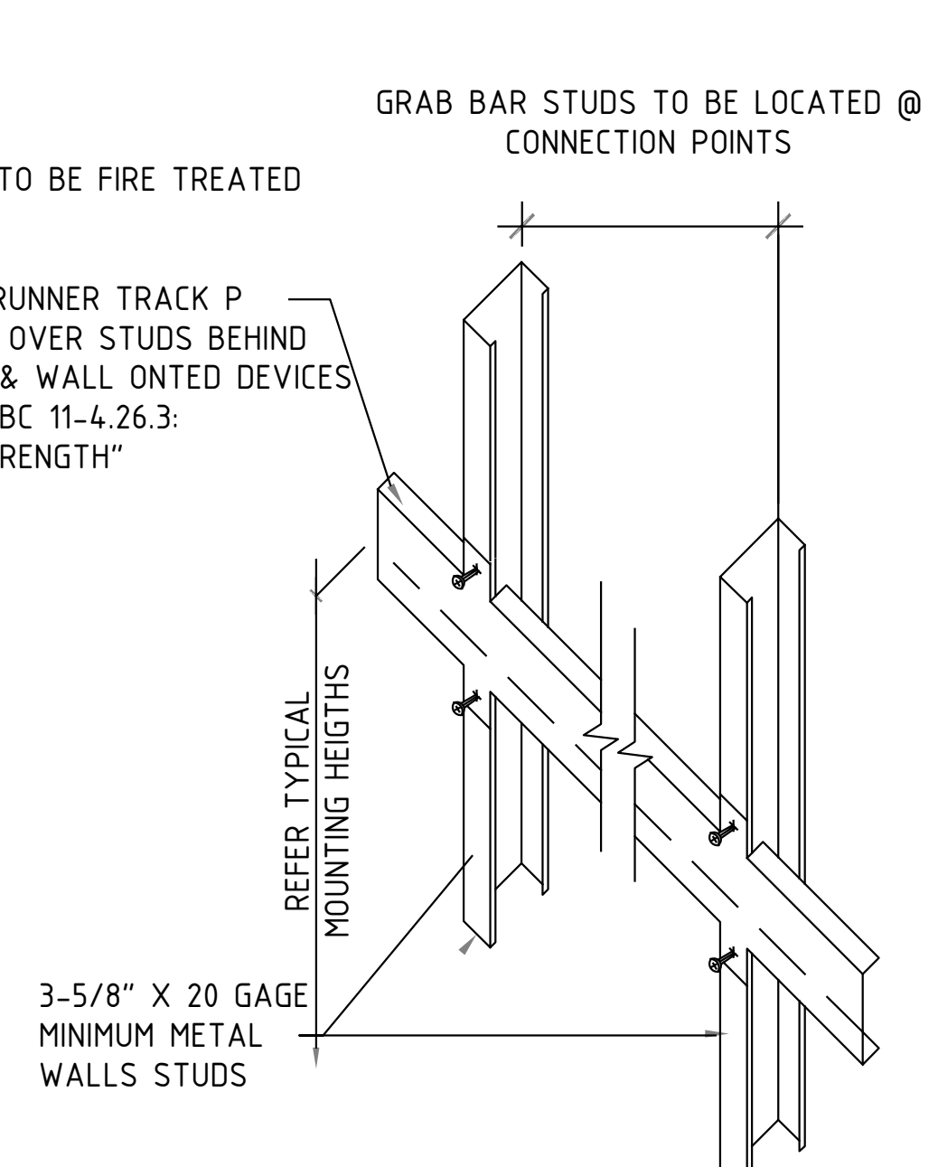
⑥ TYPICAL SUPPORT DETAIL SCALE: 1/2" = 1'-0"
