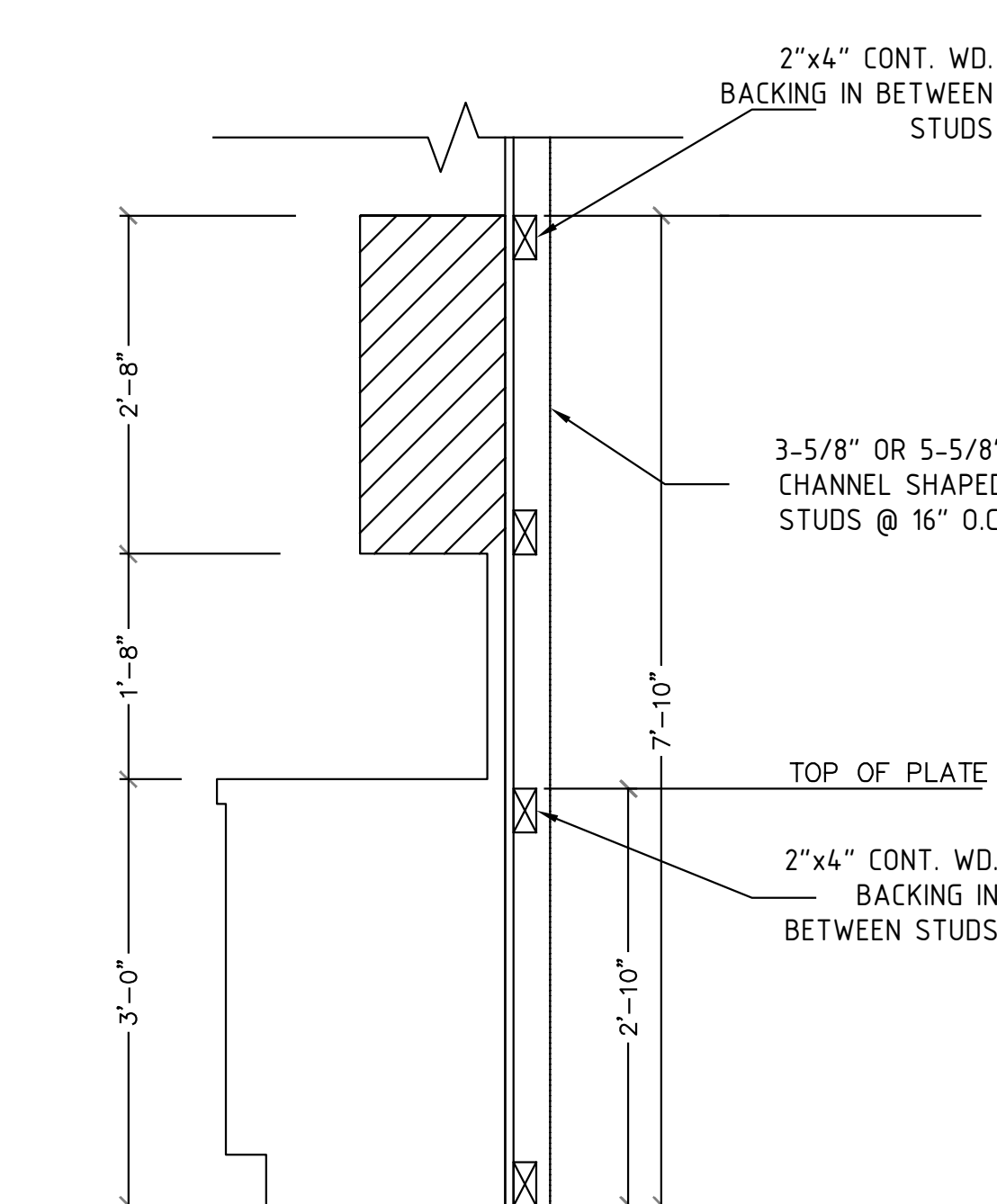
⑪ KITCHEN BACKING DETAIL SCALE: 3/4" = 1'-0"
