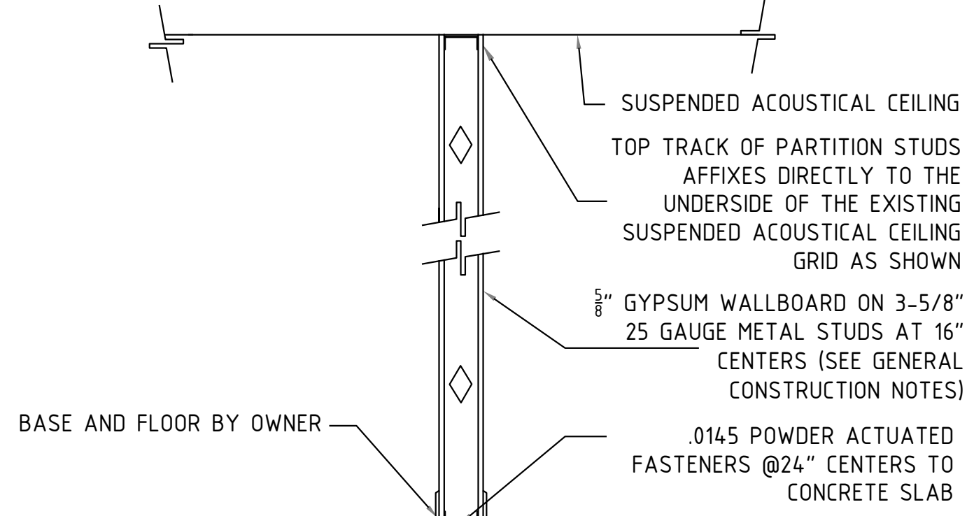
④ TYPICAL INTERIOR PARTITION SCALE: 3/8" = 1'-0" (NON-BEARING, NON- FIRE-RATED)
