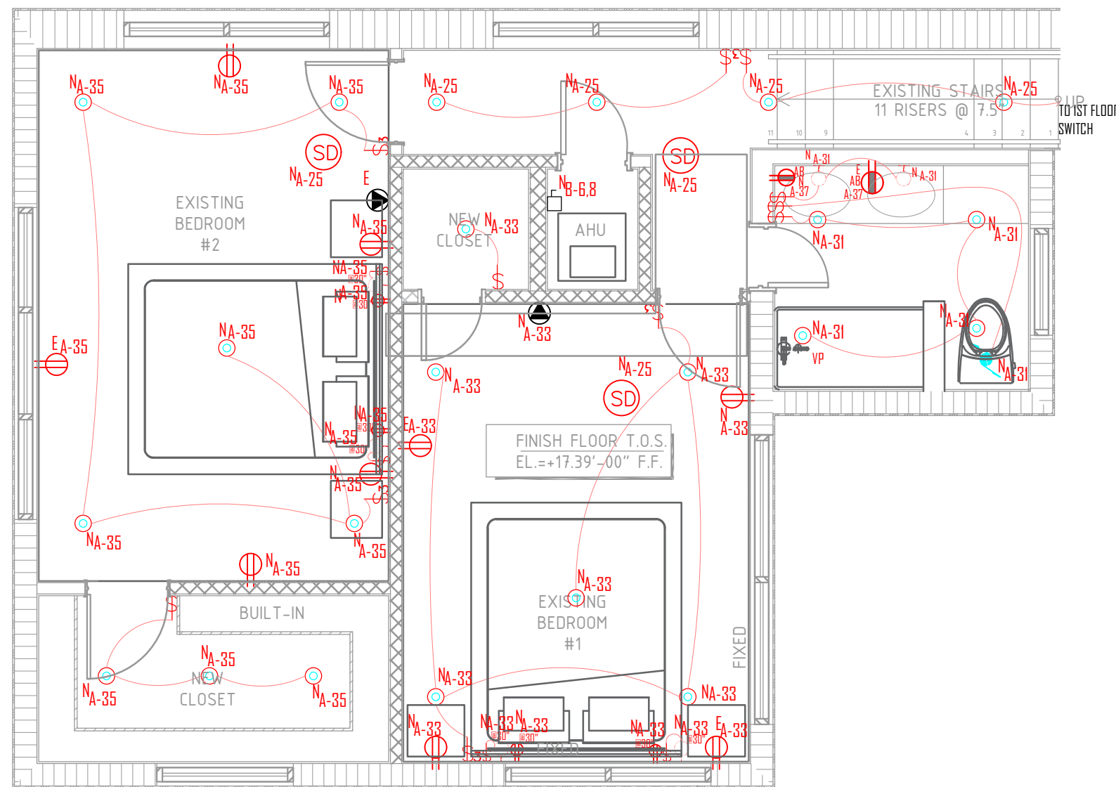
ELECTRICAL 1ST FLOOR PLAN SCALE: 1/4" = 1'-0"
